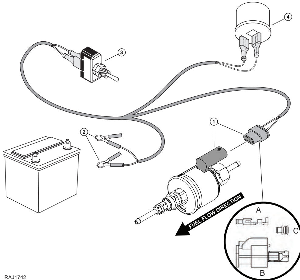
Figure 31. Heater Fuel Pump Priming Harness Connections.
