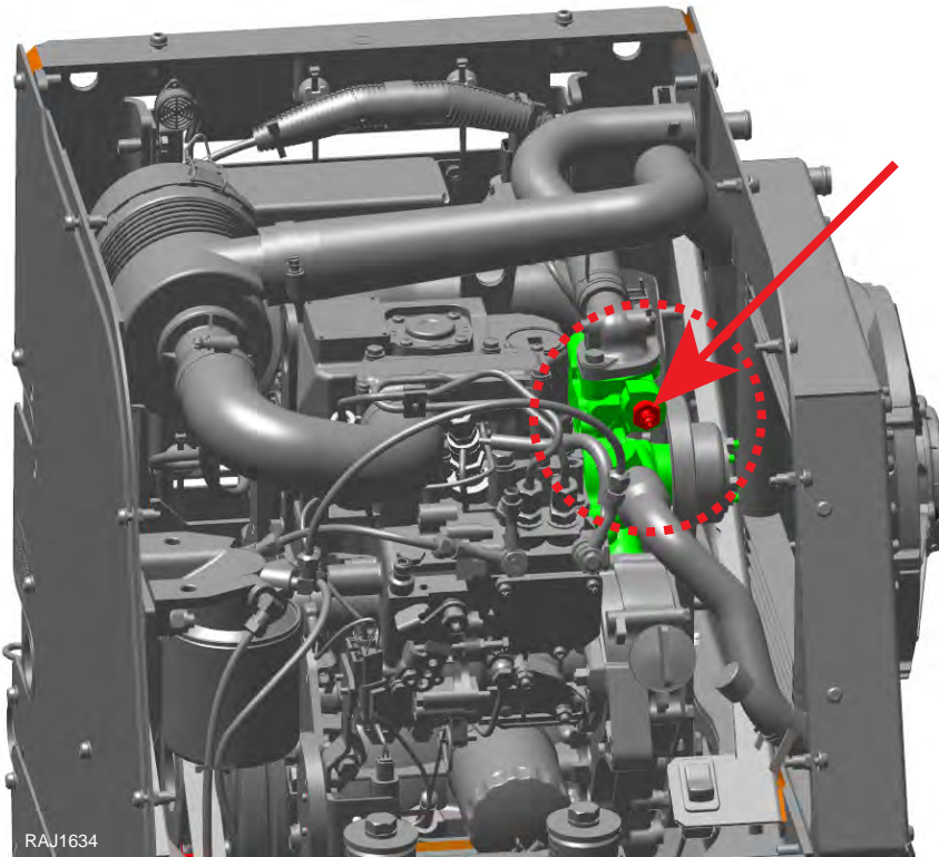
Figure 32. Coolant Bleed Valve Location On Water Pump
