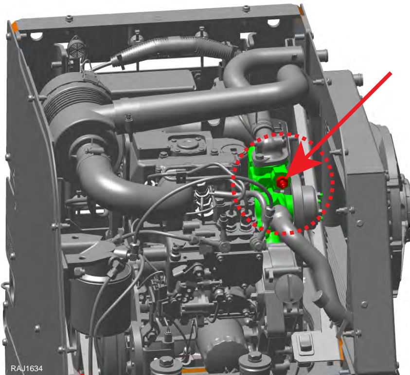
Figure 33. Coolant Bleed Valve Location On Water Pump
